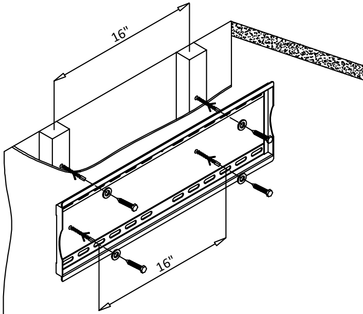
Figure 2 - Wooden Stud/Concrete Mounting
