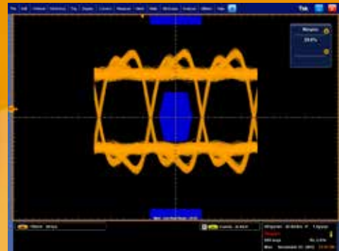
EHD-HD5M EYE PATTERN PERFORMANCE SIGNATURE
