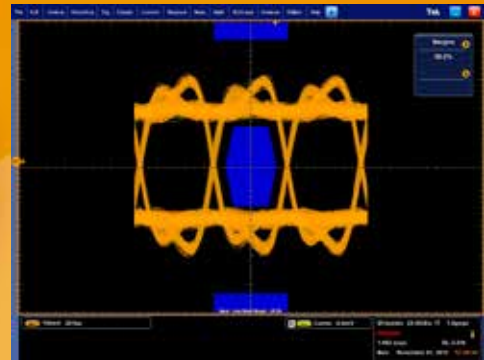
EHD-HD3M EYE PATTERN PERFORMANCE SIGNATURE
