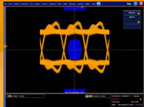
EHD-HD EYE PATTERN PERFORMANCE SIGNATURE
