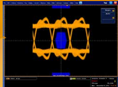
EHD-HD EYE PATTERN PERFORMANCE SIGNATURE
