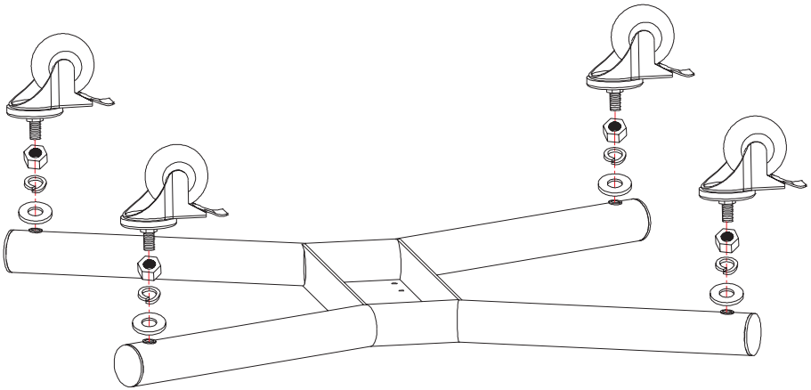
Figure 1 - Attach Wheels to Base
