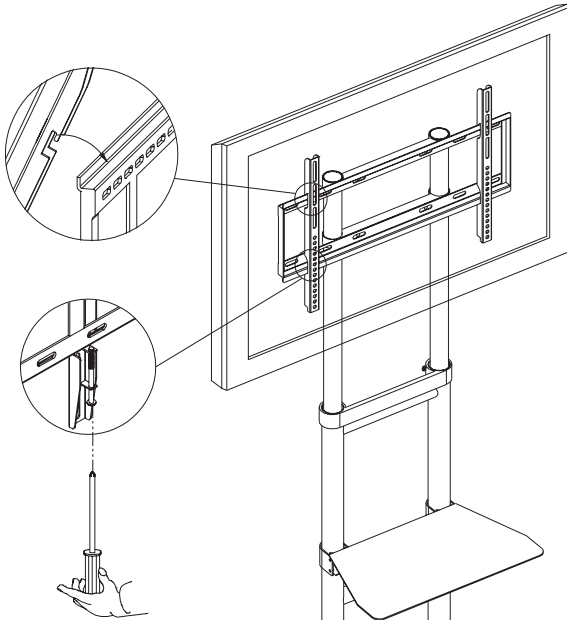
Figure 8 - Attach TV Assembly to Mounting Plate
