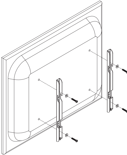
Figure 6 - Attach Brackets to TV or Audio Mount™
