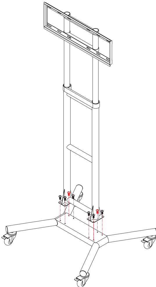
Figure 3 - Attach Pole to Base
