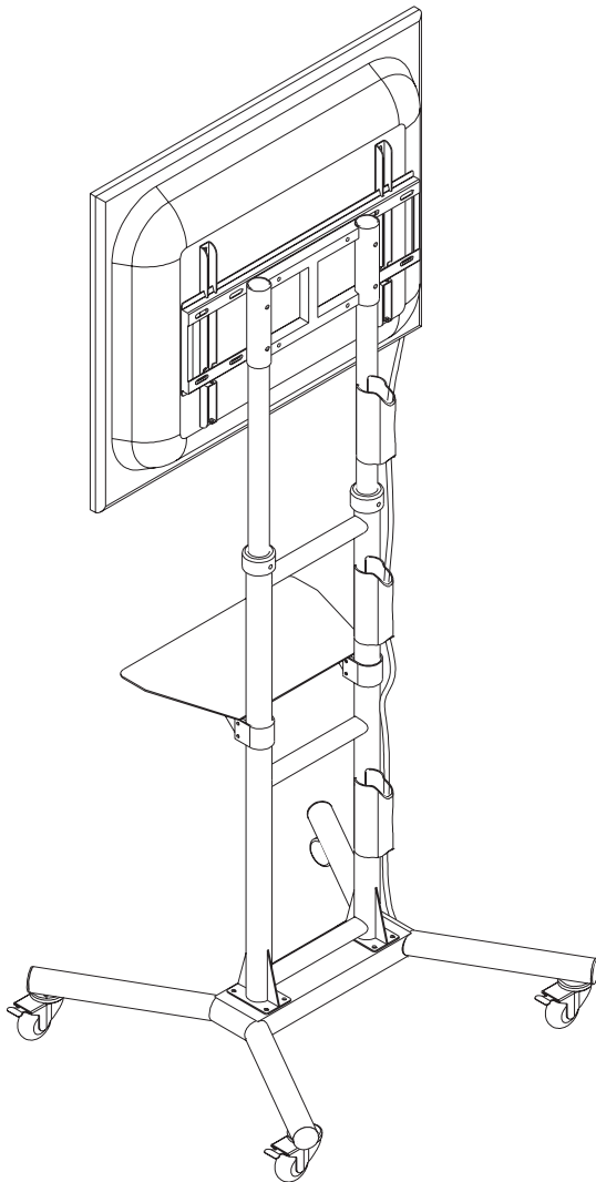
Figure 9 - Route and Secure Cables
