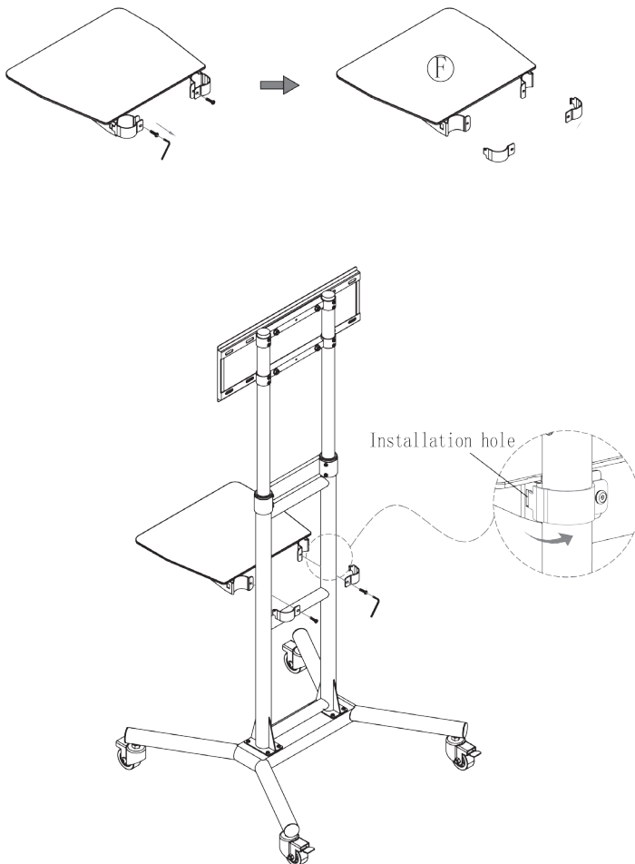
Figure 5 - Install Metal Tray
