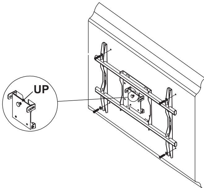
Figure 3 - Attach Brackets to TV
