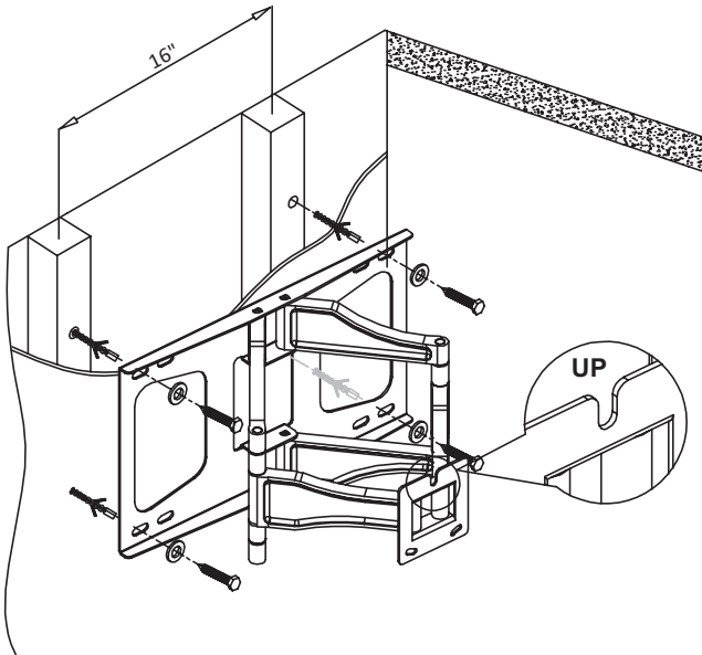
Figure 2 - Wood Stud/Concrete Mounting
