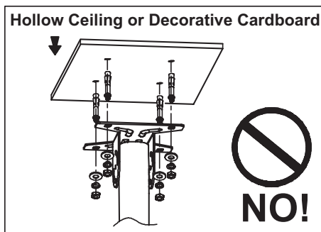
Figure 1 - Hollow Ceiling WARNING!
