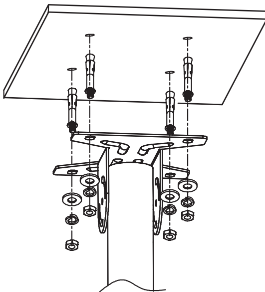
Figure 2 - Concrete Mounting
