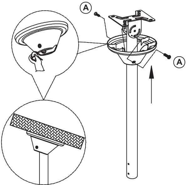
Figure 3 - Secure Plastic Cover Over Ceiling Plate
