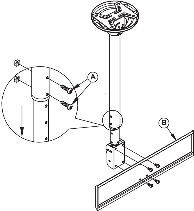
Figure 4 - Adjust Height/Install Front Plate
